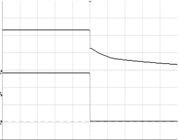
Figure 7 Output voltage shut down by power off, (200ms/div), see Figure 11 for test configuration, CH1-input voltage (20V/div); CH2-output voltage (10V/div)
