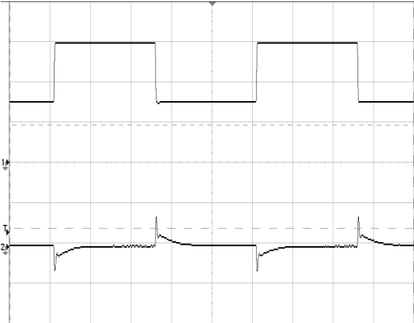
Figure 4 Dynamic response for 25% load step (25% ~ 50% ~ 25%) and 0.1A/ \mu s slew rate, see Figure 11 for test configuration, CH2-output voltage (500mV/div); CH1-output current (5A/div)
