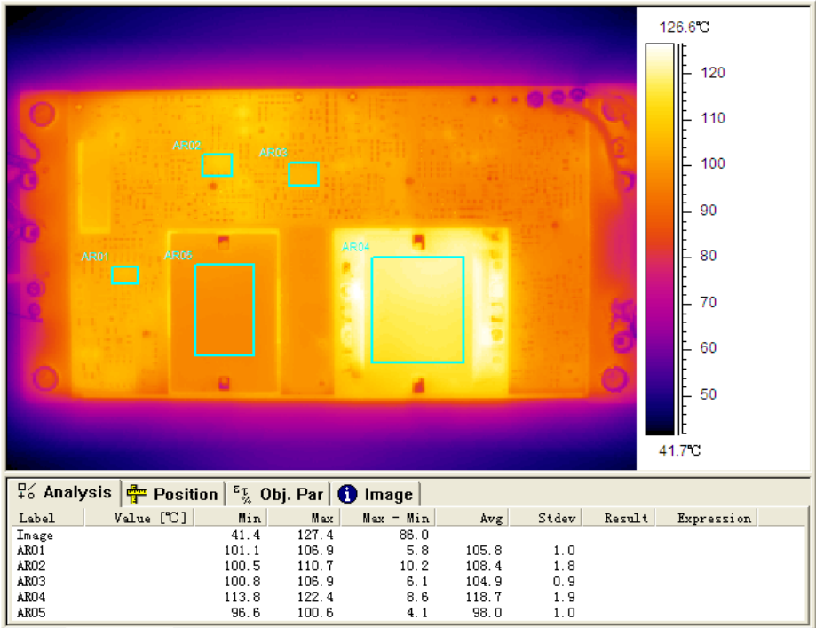
Figure 21 Thermal image, 48V in , 28V o , full load, room temperature
