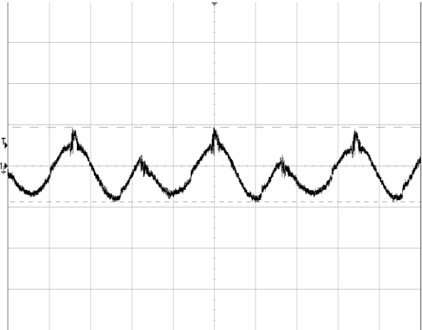
Figure 3 Input reflected ripple current (2 \mu\text{s}/\text{div} , 20mA/div), see Figure 16 for test configuration
