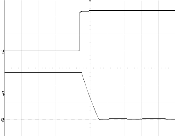
Figure 9 Output voltage shutdown by remote OFF, (1ms/div), see Figure 12 for test configuration, CH1-remote OFF (20V/div); CH2-output voltage (10V/div)
