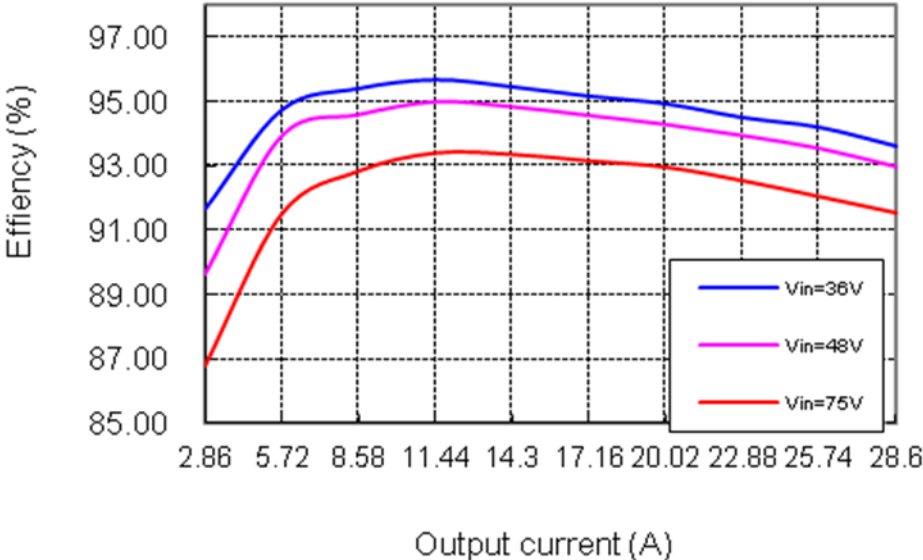
Figure 1 Efficiency vs. output current, T_a=25^{\circ}\text{C} , T_c=40^{\circ}\text{C} , V_o=28\text{V}
