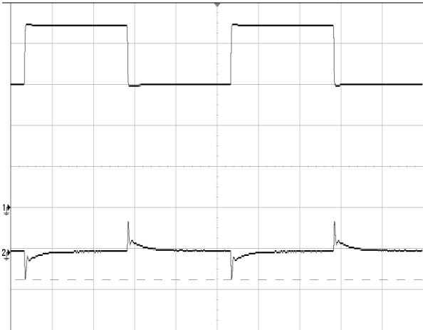
Figure 5 Dynamic response for 25% load step (50% ~ 75% ~ 50%) and 0.1A/ \mu s slew rate, see Figure 11 for test configuration. CH2-output voltage (500mV/div); CH1-output current (5A/div)
