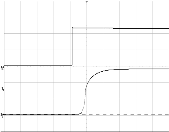
Figure 6 Output voltage startup by power on, (200ms/div), see Figure 11 for test configuration, CH1-input voltage (20V/div); CH2-output voltage (10V/div)
