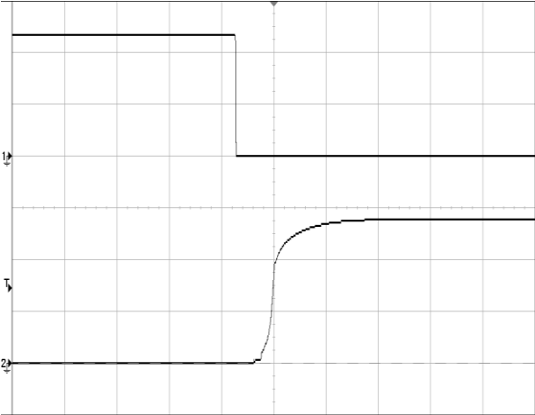
Figure 8 Output voltage startup by remote ON, (200ms/div), see Figure 12 for test configuration, CH1-remote ON (20V/div); CH2-output voltage (10V/div)
