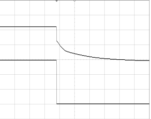
Figure 7 Output voltage shutdown by power off, (500ms/div), see Figure 11 for test configuration, CH1-input voltage (20V/div); CH2-output voltage (10V/div)
