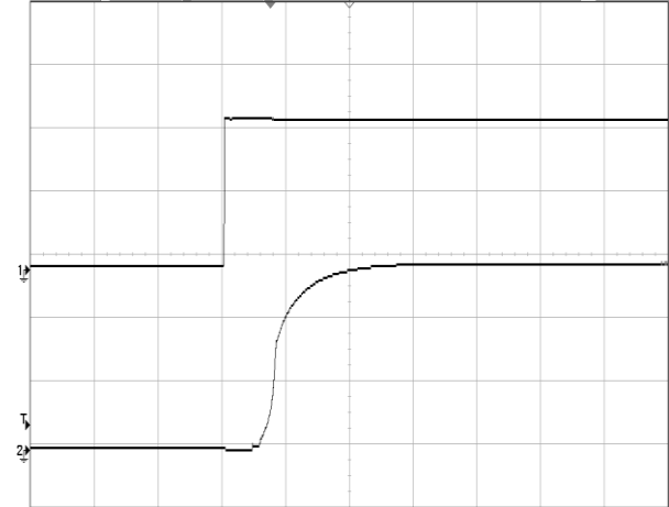
Figure 6 Output voltage startup by power on, (200ms/div), see Figure 11 for test configuration, CH1-input voltage (20V/div); CH2-output voltage (10V/div)
