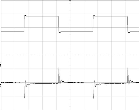
Figure 5 Dynamic response for 25% load step (50% ~ 75% ~ 50%) and 0.1A/μs slew rate, see Figure 11 for test configuration. CH1-output voltage (200mV/div); CH2-output current (5A/div)
