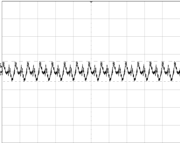
Figure 2 Output ripple & noise (10 \mu\text{s}/\text{div} , 100mV/div), see Figure 16 for test configuration
