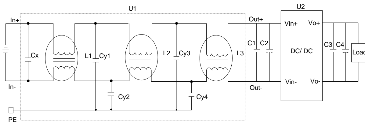
Figure 17 EMC test configuration
