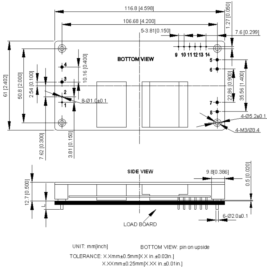
Figure 18 Mechanical diagram
