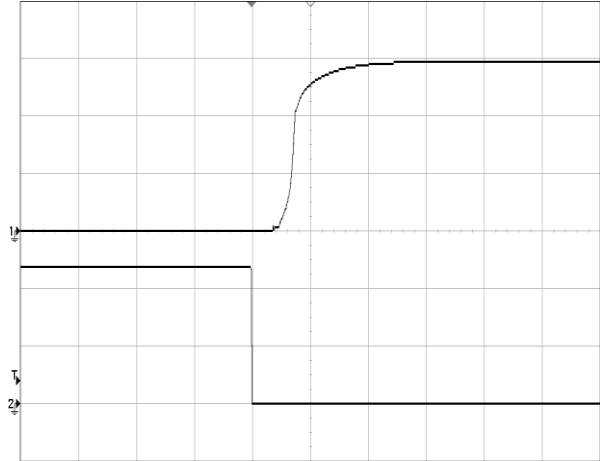
Figure 8 Output voltage startup by remote ON, (200ms/div), see Figure 12 for test configuration, CH2-remote ON (20V/div); CH1-output voltage (10V/div)
