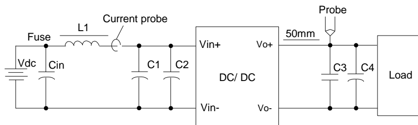
Figure 16 Ripple & noise test configuration
