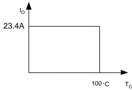
Figure 20 Output power derating curve, T_c : temperature test point on baseplate, see Figure 19
