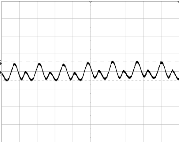
Figure 3 Input reflected ripple current (5 \mu\text{s}/\text{div} , 20mA/div), see Figure 16 for test configuration
