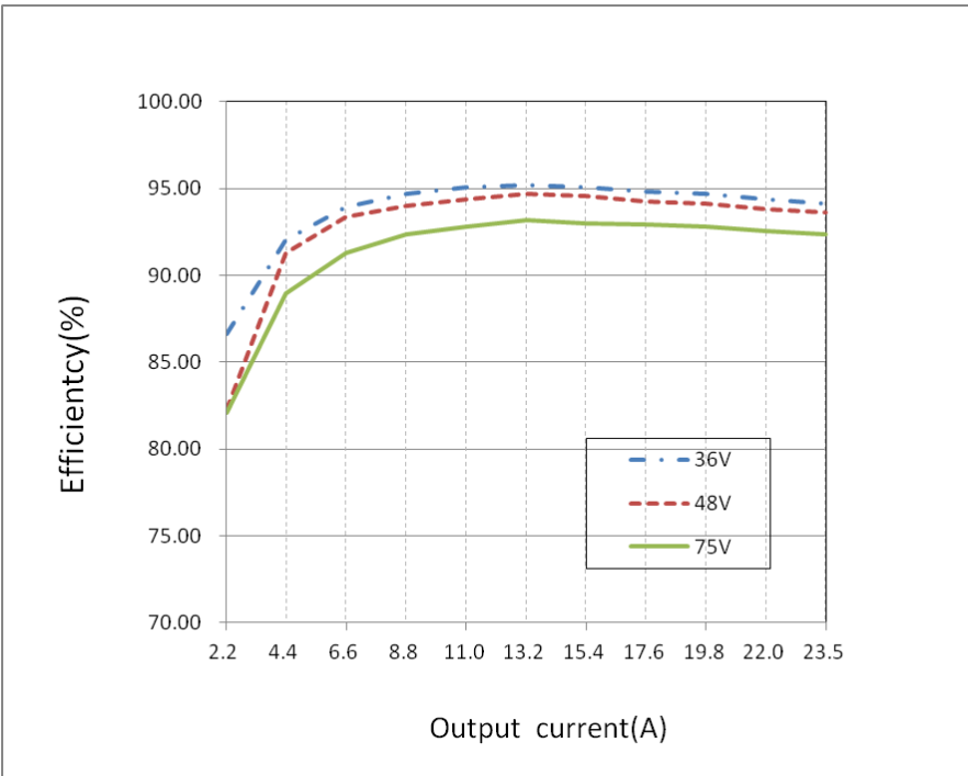
Figure 1 Efficiency vs. output current, T_a = 25^\circ\text{C} , T_c = 40^\circ\text{C} , V_o = 30\text{V}
