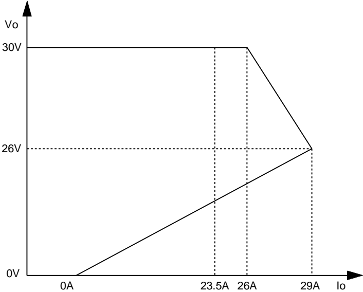
Figure 10 Over-current protection characteristics
