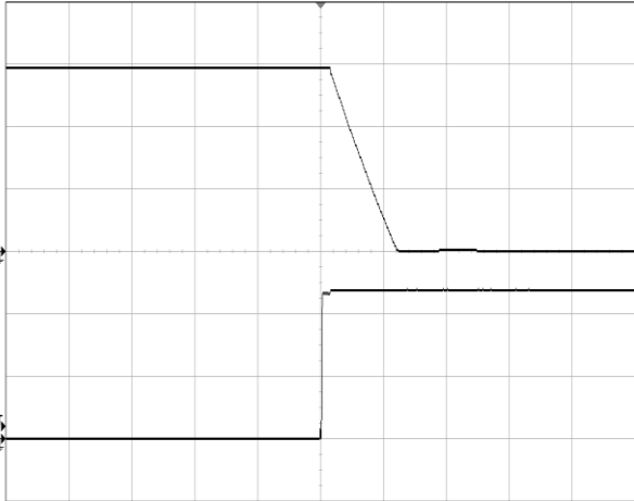
Figure 9 Output voltage shutdown by remote OFF, (1ms/div), see Figure 12 for test configuration, CH2-remote OFF (20V/div); CH1-output voltage (10V/div)
