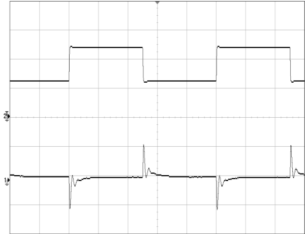
Figure 4 Dynamic response for 25% load step (25% ~ 50% ~ 25%) and 0.1A/μs slew rate, see Figure 11 for test configuration. CH1-output voltage (200mV/div); CH2-output current (5A/div)
