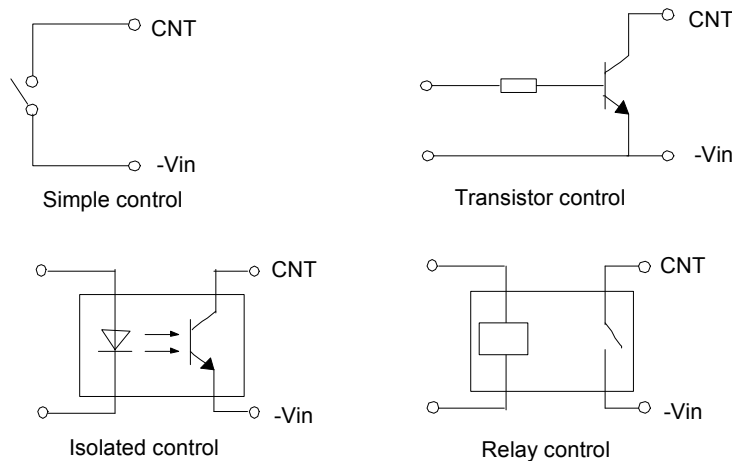
Figure 11 Remote ON/OFF internal diagram
