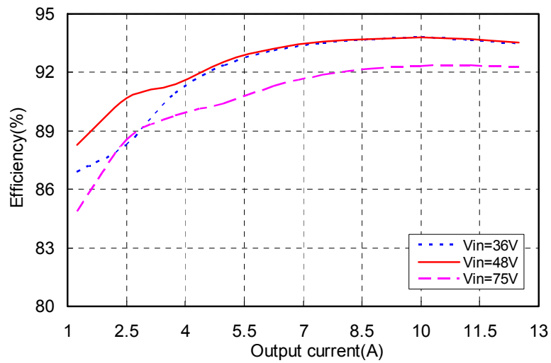
Figure 1 Efficiency vs. output current, T_a=25^{\circ}\text{C} , T_c<40^{\circ}\text{C} , V_o=28\text{V} T_c : temperature test point on baseplate, see Figure 18 for test configuration
