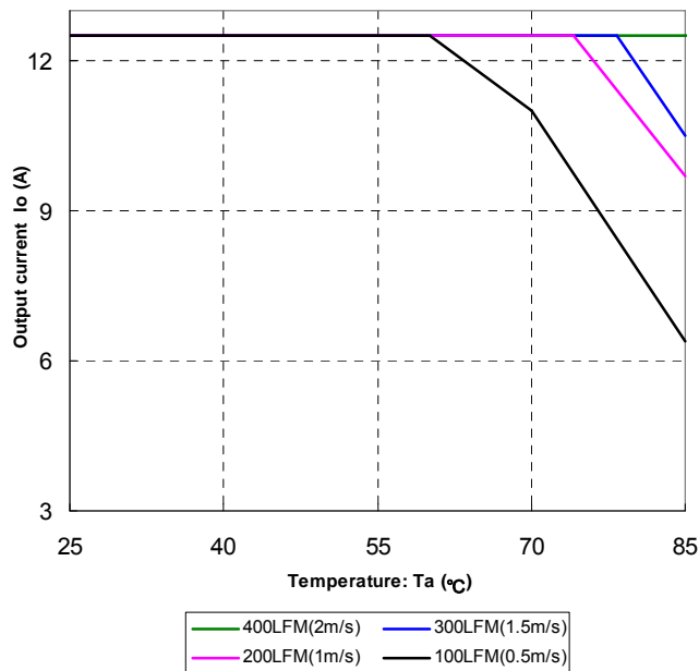
Figure 20 Output power derating, 48Vin
