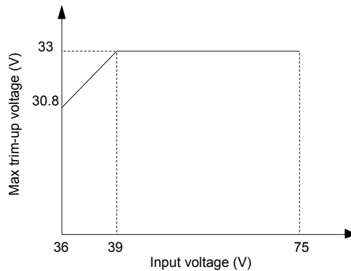
Figure 14 Max trim-up voltage vs. input voltage
