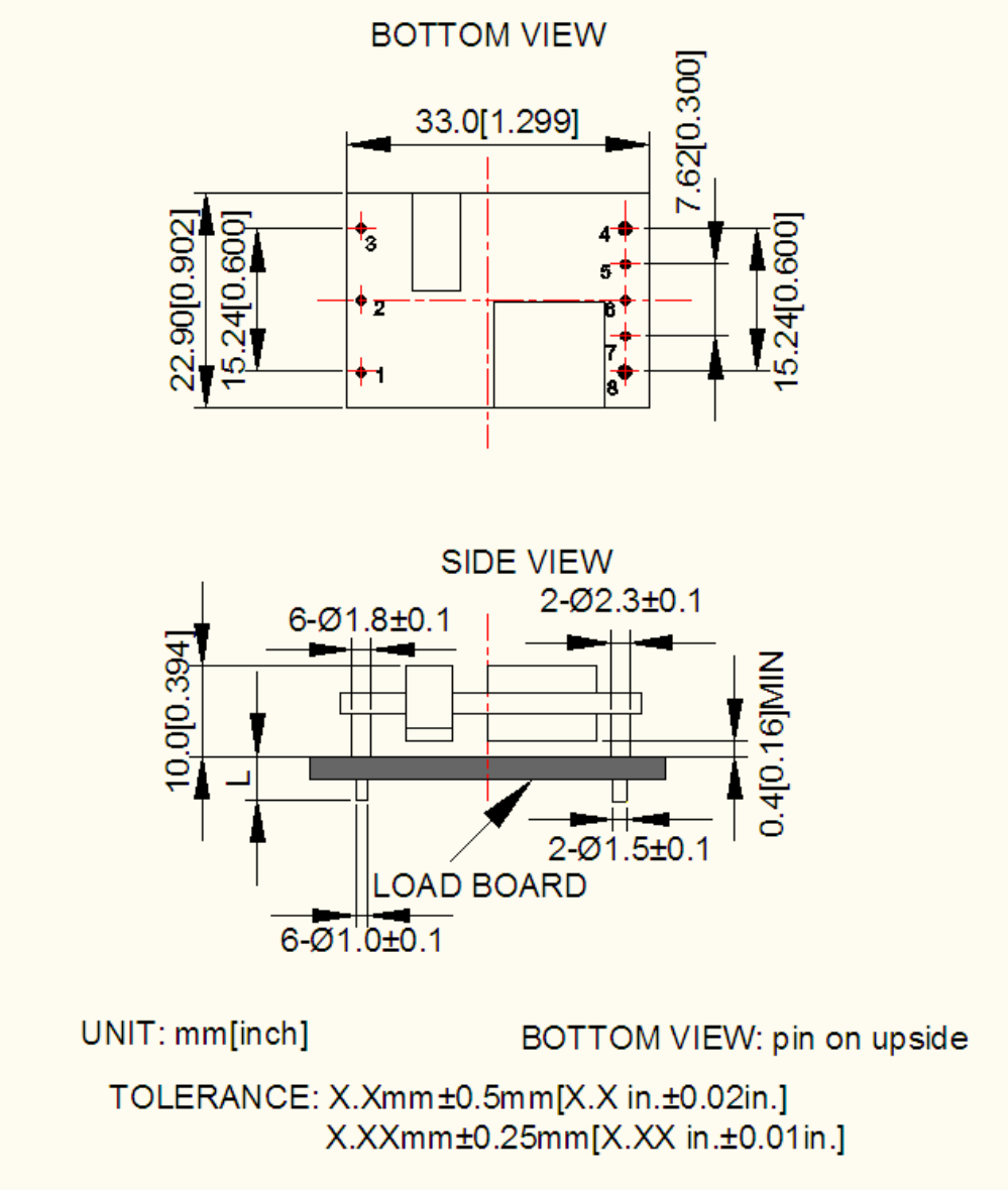
open Frame Module Mechanical diagram
