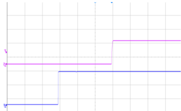
Figure 6 Output voltage startup by power on, (20ms/div), see Figure 11 for test configuration; CH1-input voltage (20V/div);CH2-output voltage (2V/div)
