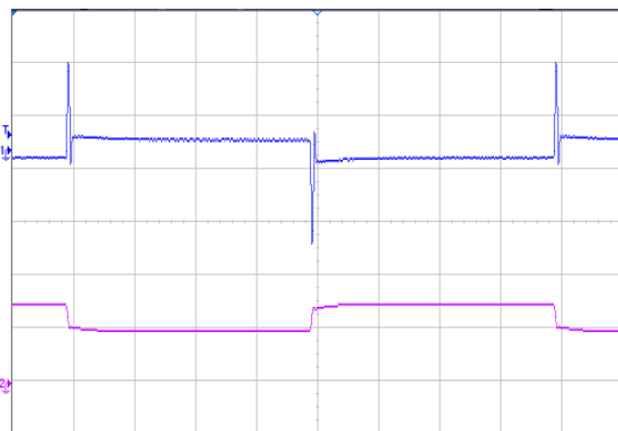
Figure 4 Dynamic response for 25% load step (50% ~ 75% ~ 50%) and 0.1A/ \mu\text{s} slew rate, (1ms/div), see Figure 11 for test configuration; CH2-output current (10A/div);CH1-output voltage (10mV/div)
