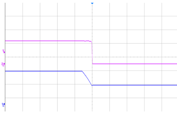
Figure 7 Output voltage shut down by power off, (100ms/div), see Figure 11 for test configuration; CH1-input voltage (20V/div);CH2-output voltage (2V/div)
