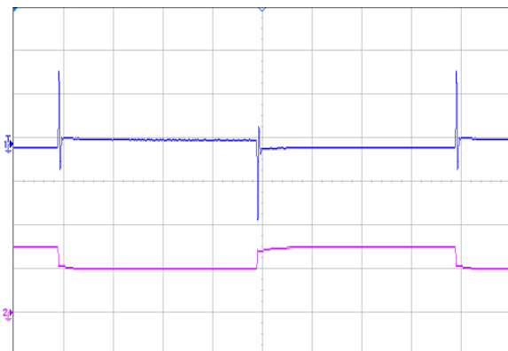
Figure 5 Dynamic response for 25% load step (50% ~ 75% ~ 50%) and 1A/ \mu\text{s} slew rate(1ms/div), see Figure 11 for test configuration; CH2-output current (10A/div);CH1-output voltage (20mV/div)
