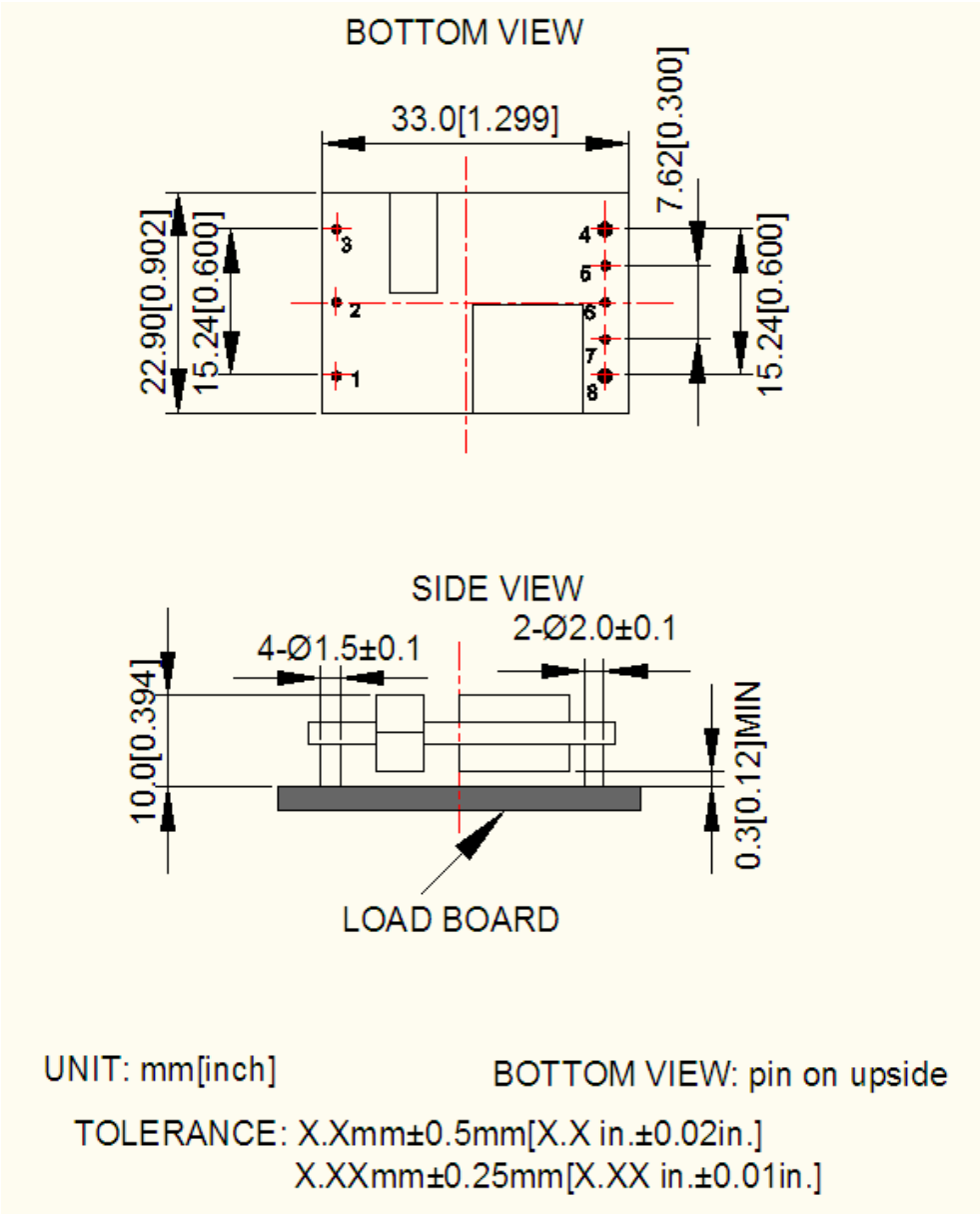
open Frame Module with SMT pin Mechanical diagram
