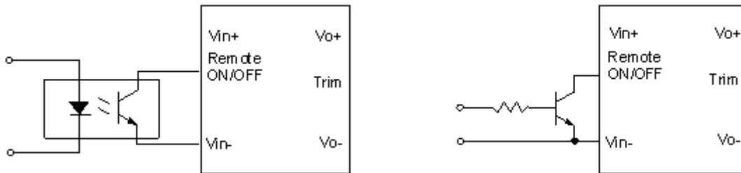
Isolated remote ON/OFF circuit
