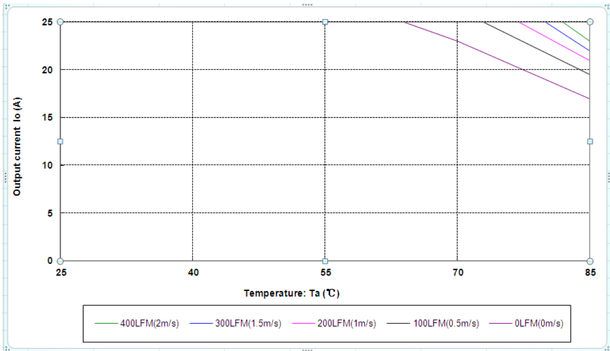
Figure 18 Output power derating, 48Vin, air flowing across the converter (from pin 3 to pin1)
