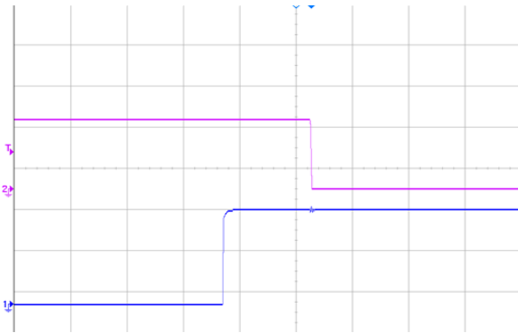
Figure 9 Output voltage shutdown by remote OFF, (50ms/div), see Figure 11 for test configuration; CH1-remote ON (2V/div);CH2-output voltage (2V/div)
