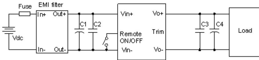
Figure 11 Typical application
