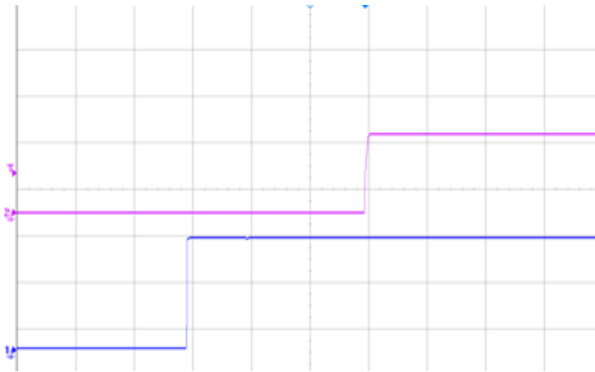
Figure 6 Output voltage startup by power on, (20ms/div), see Figure 11 for test configuration; CH1-input voltage (20V/div);CH2-output voltage (2V/div)
