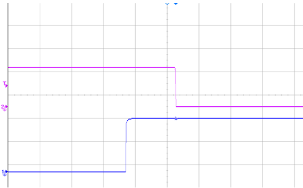
Figure 9 Output voltage shutdown by remote OFF, (50ms/div), see Figure 11 for test configuration; CH1-remote ON (2V/div);CH2-output voltage (2V/div)
