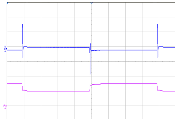
Figure 5 Dynamic response for 25% load step (50% ~ 75% ~ 50%) and 1A/ \mu\text{s} slew rate, (1ms/div), see Figure 11 for test configuration; CH2-output current (10A/div);CH1-output voltage (10mV/div)
