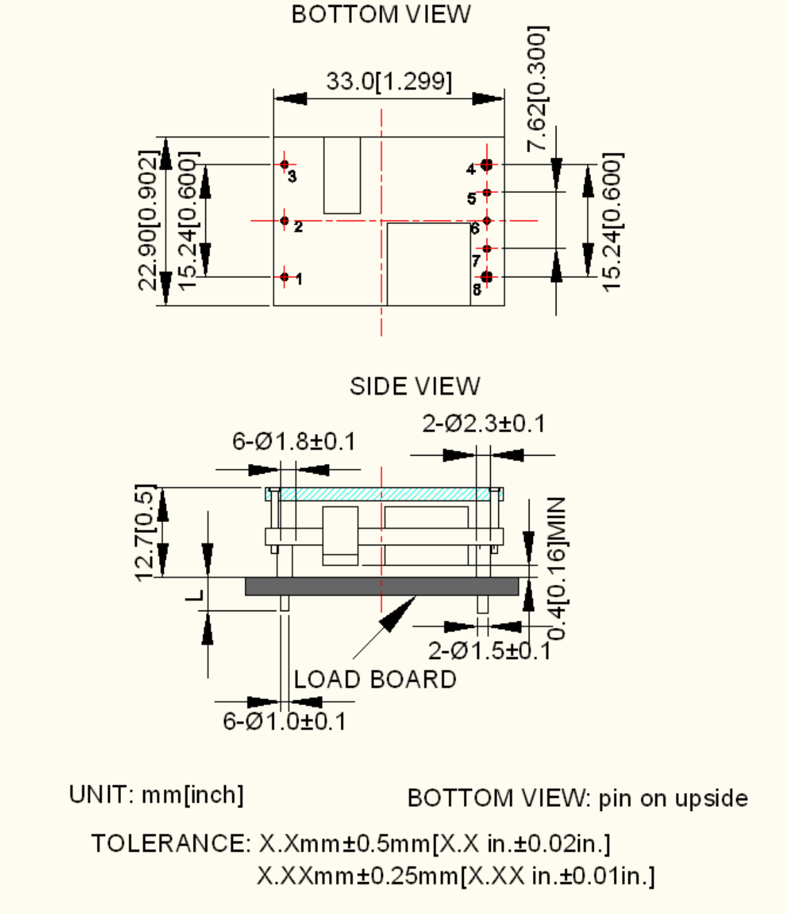
Mechanical diagram with base plate
