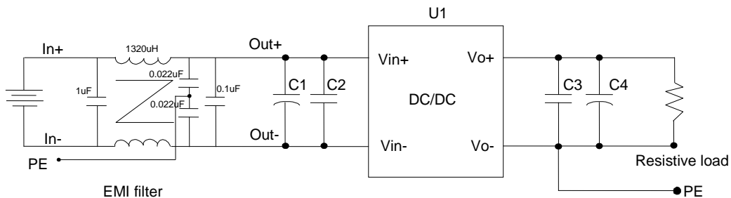
Figure 16 EMC test configuration
