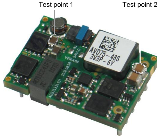
Temperature test point on FR-4 board
