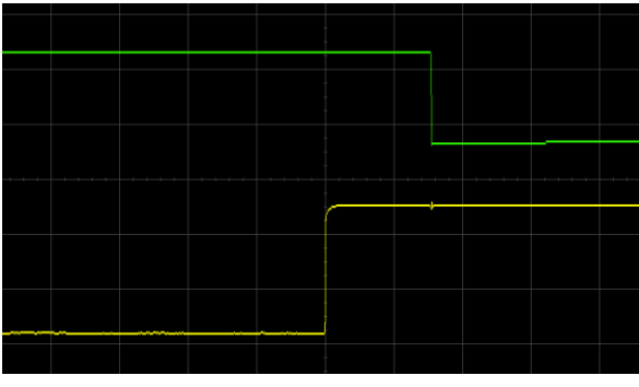
Figure 9 Output voltage shutdown by remote OFF, (10ms/div) ,see Figure 11 for test configuration; CH1-remote ON (2V/div);CH2-output voltage (2V/div)
