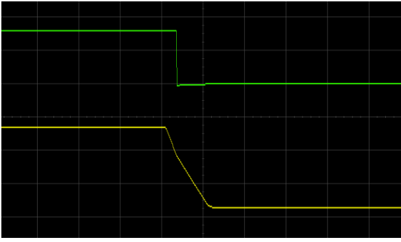
Figure 7 Output voltage shut down by power off, (100ms/div), see Figure 11 for test configuration; CH1-input voltage (20V/div);CH2-output voltage (2V/div)
