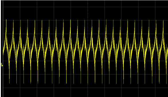
Figure 2 Output ripple & noise (5 \mu\text{s}/\text{div} , 20mV/div), see Figure 15 for test configuration
