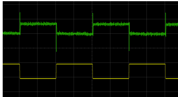
Figure 5 Dynamic response for 25% load step (50% ~ 75% ~ 50%) and 1A/ \mu\text{s} slew rate, (1.0ms/div), see Figure 11 for test configuration; CH1-output current (5A/div);CH2-output voltage (20mV/div)
