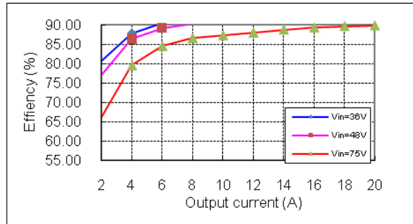
Figure 1 Efficiency vs. output current, T_a=25^{\circ}\text{C} , 200LFM, V_o=3.3\text{V}
