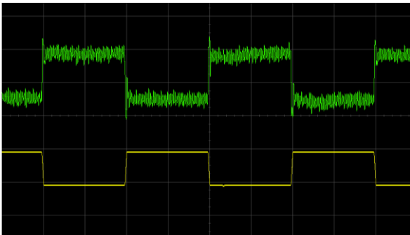
Figure 4 Dynamic response for 25% load step (50% ~ 75% ~ 50%) and 0.1A/ \mu\text{s} slew rate, (1ms/div), see Figure 11 for test configuration; CH1-output current (5A/div);CH2-output voltage (10mV/div)
