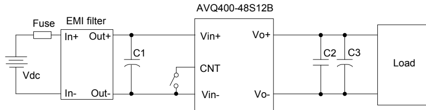
Figure 11 Typical application
