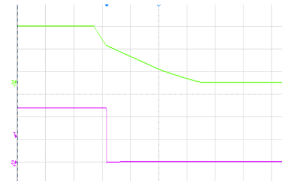
Figure 7 Output voltage shut down by power off, (100ms/div), see Figure 11 for test configuration; CH2-output voltage (5V/div); CH3-input voltage (20V/div)
