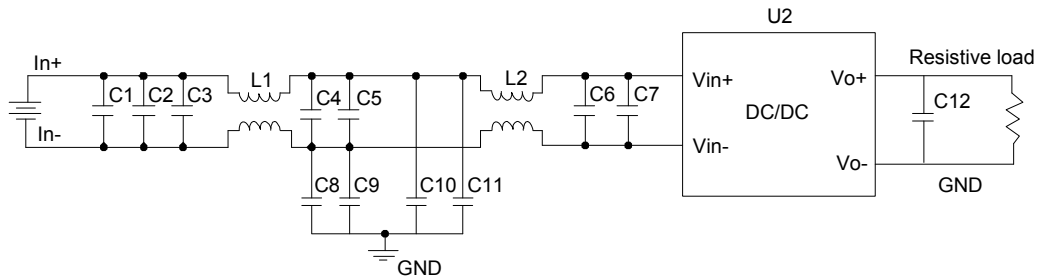
Figure 15 EMC test configuration
