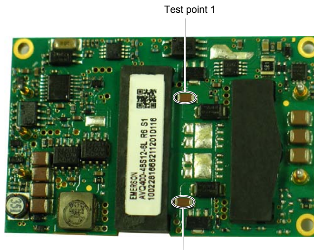
Temperature test points on FR-4 board
