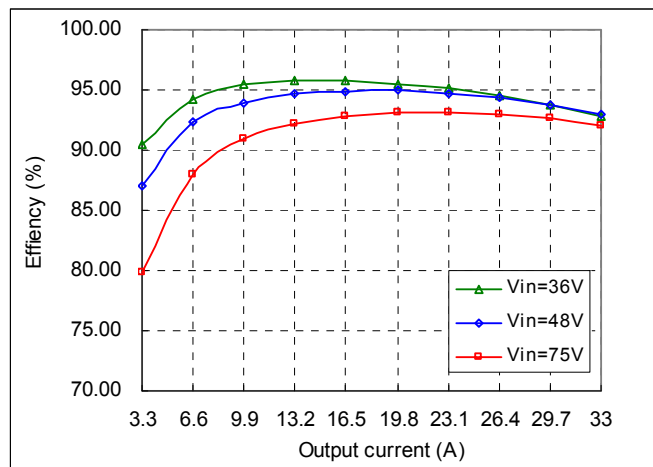
Figure 1 Efficiency and output current, T_a = 25^{\circ}\text{C} , 400LFM, V_o = 12\text{V}
