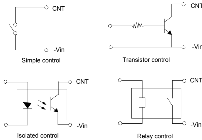
Figure 13 External remote ON/OFF circuit
