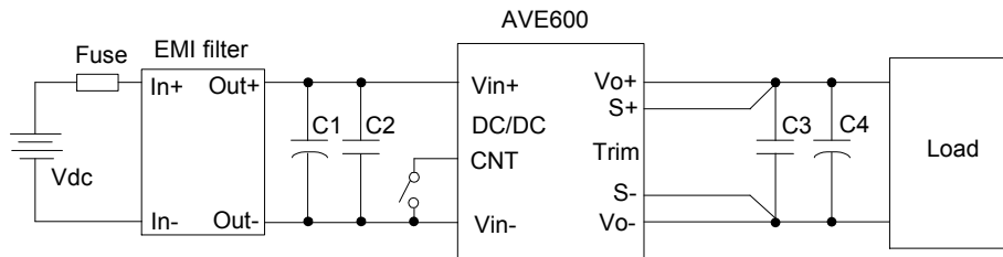
Figure 11 Typical application
