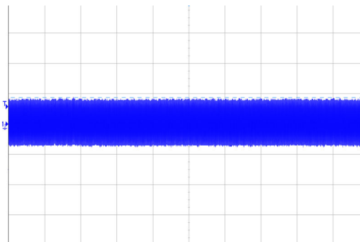
Figure 3 Input reflected ripple current (100ms/div, 50mA/div), see Figure 17 for test configuration
