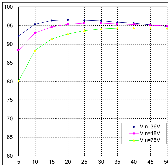
Figure 1 Efficiency and output current, T_a = 25^\circ\text{C} , V_o = 12\text{V}
