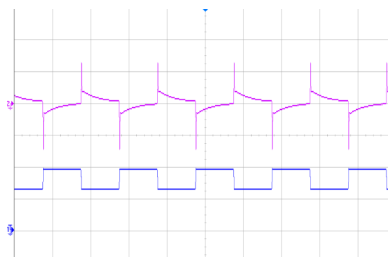
Figure 5 Dynamic response for 25% load step (50% ~ 75% ~ 50%) and 1A/ \mu\text{s} slew rate, (5ms/div), see Figure 11 for test configuration; CH2-output voltage (200mV/div); CH1-output current (20A/div)
