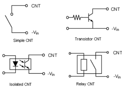
Fig.7 CNT circuits
