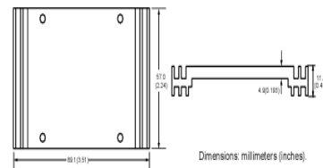
Figure 23 Non-standard heatsink
