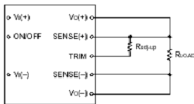
Figure 9 Trim up circuit
