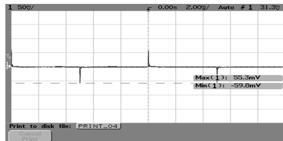
Fig4 AVE300-48S1V2-4. Typical Transient Response to Ta:25 , Air velocity: 300LFM, forced air direction: from Vin+ to Vin-. Vin: 48V, Vonom, 50% Ionom step from 75% Ionom, 0.1A/μs , the external capacitor should be “10μ tantalum(ESR 100 mΩ) // 1μ ceramic capacitor.
