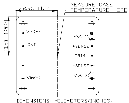
Figure 18 Temperature measurement location (with baseplate)
