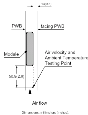
Figure 20 Experiment setup
