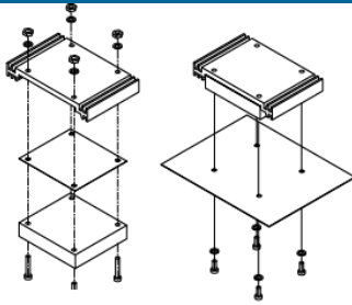
Figure 26 Heatsink mounting
