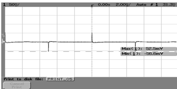
Fig3 AVE300-48S1V2-4 Typical Transient Response to Ta:25 , Air velocity: 300LFM, forced air direction: from Vin+ to Vin-. Vin: 48V, Vonom, 25% Ionom step from 50% Ionom, 0.1A/μs , the external capacitor should be “10μ tantalum(ESR 100 mΩ) // 1μ ceramic capacitor.
