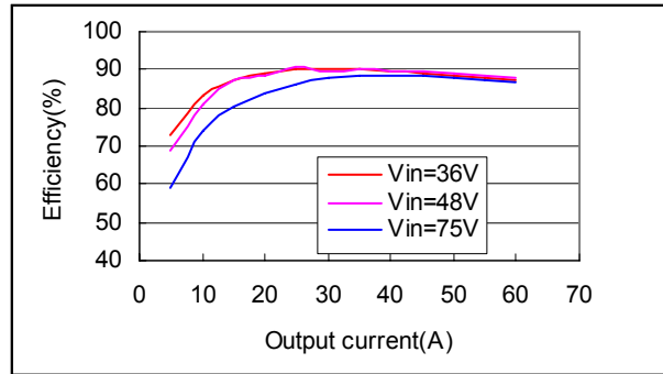
Fig.1 AVE300-48S1V5-4 Typical Efficiency
