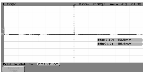
Fig3 AVE300-48S1V5-4 Typical Transient Response to Ta:25°C, Air velocity: 300LFM, forced air direction: from Vin+ to Vin-. Vin: 48V, Vonom, 25% Ionom step from 50% Ionom, 0.1A/µs”, the external capacitor should be “10µ tantalum(ESR≤100 mΩ) // 1µ ceramic capacitor.
