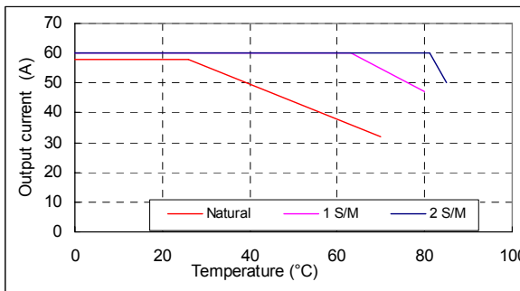
Figure 22 Forced convection power derating with baseplate
