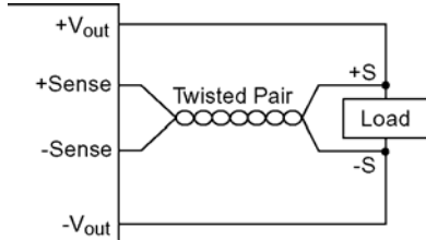
Figure 8 Sense connection
