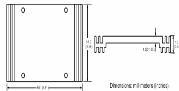
Figure 23 Non-standard heatsink
