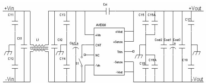
Figure 17 EMI reduction filter
