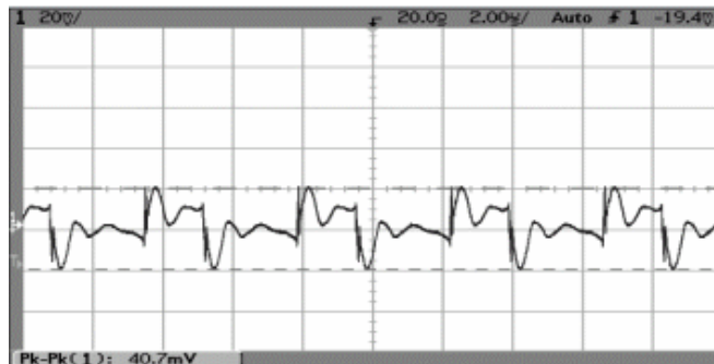
Fig.2 AVE300-48S1V5-4 Typical Output Ripple Voltage
