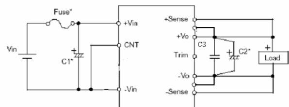
Fig 15 Typical application
