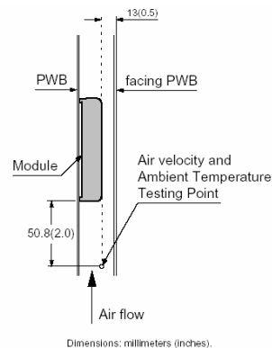
Figure 20 Experiment setup
