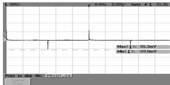
Fig4 AVE300-48S1V5-4. Typical Transient Response to Ta:25°C, Air velocity: 300LFM, forced air direction: from Vin+ to Vin-. Vin: 48V, Vonom, 50% Ionom step from 75% Ionom, 0.1A/µs”, the external capacitor should be “10µ tantalum(ESR≤100 mΩ) // 1µ ceramic capacitor.
