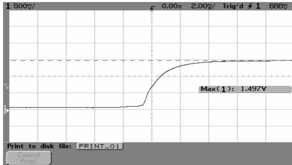
Fig.5 Typical start-up from power on
