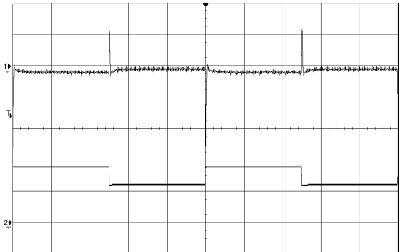
Figure 5 Dynamic response for 25% load step (50% ~ 75% ~ 50%) and 1A/ \mu s slew rate, (2ms/div), see Figure 11 for test configuration; CH1-output voltage (50mV/div); CH2-output current (2A/div)
