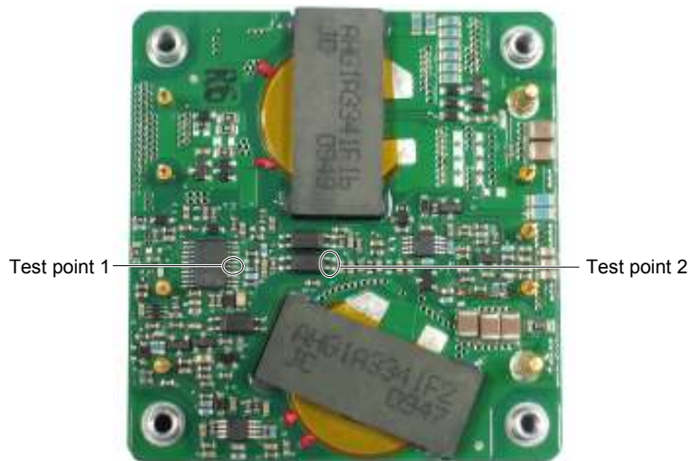
Figure 18 Temperature test points
