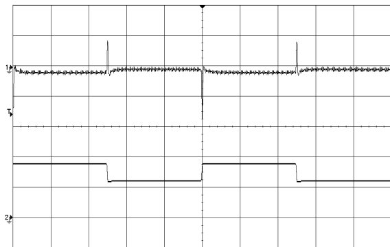
Figure 4 Dynamic response for 25% load step (50% ~ 75% ~ 50%) and 0.1A/ \mu s slew rate, (2ms/div), see Figure 11 for test configuration; CH1-output voltage (50mV/div); CH2-output current (2A/div)
