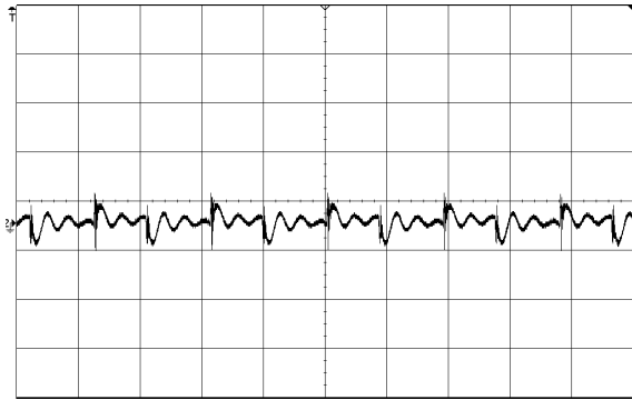
Figure 2 Output ripple & noise (2 \mu s/div, 50mV/div), see Figure 16 for test configuration
