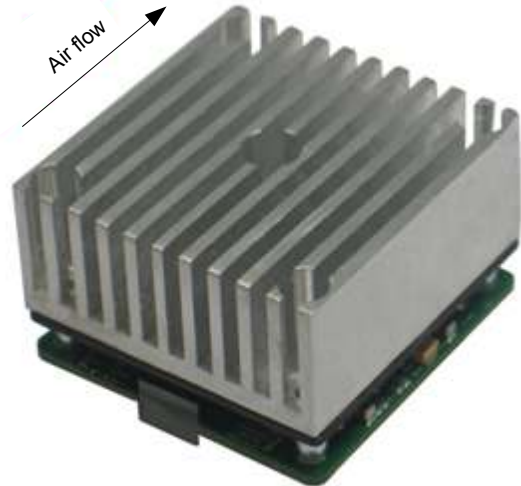
Figure 19 Typical test condition, forced airflow direction is from V_{in-} to V_{in+}
