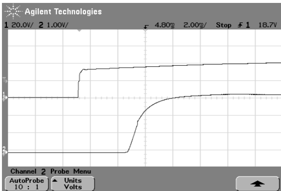
Fig.27 Typical start-up from power on of AVQ100B-48S3V3
