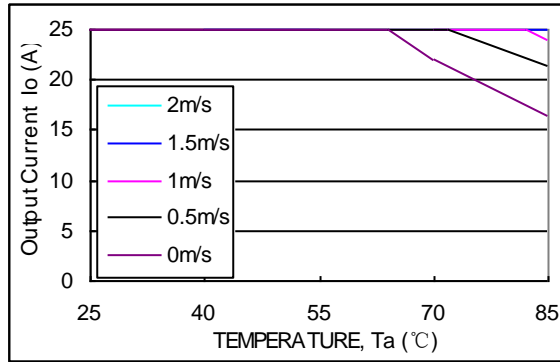
Fig.44 Output power derating AGQ100-48S1V5 (airflow direction from output to input, baseplate)
