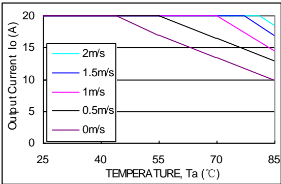
Fig.49 Output power derating AVQ100B-48S05 (airflow direction from output to input, open frame)
