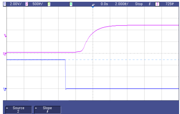
Fig.22 Typical start-up from CNT on of AGQ100-48S1V2
