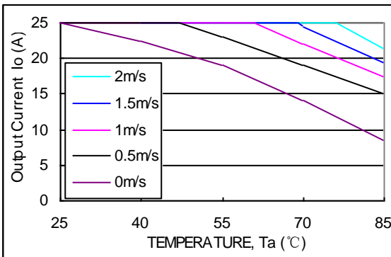
Fig.47 Output power derating AVQ100B-48S3V3 (airflow direction from output to input, open frame)
