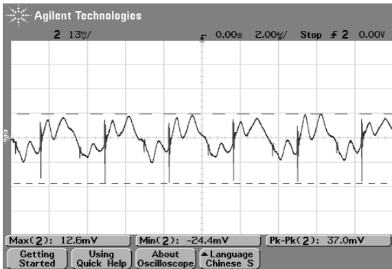
Fig. 20 Typical output ripple voltage AVQ100B -48S05, room temperature, I_o = I_{o,max}
