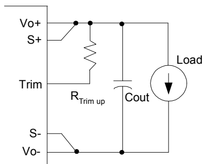
Figure 13 Trim up
