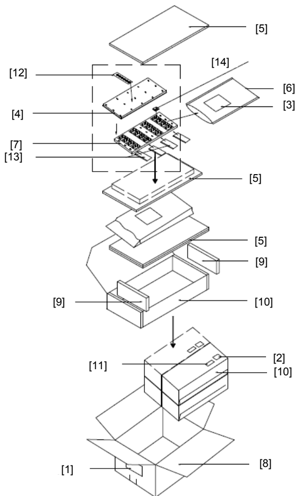
Figure 23 Package disassembly
