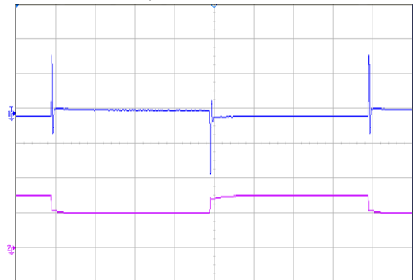
Figure 5 Dynamic response for 25% load step (50% ~ 75% ~ 50%) and 1A/ \mu\text{s} slew rate, (1ms/div), see Figure 11; CH1-output voltage (100mV/div) CH2-output current (10A/div)
