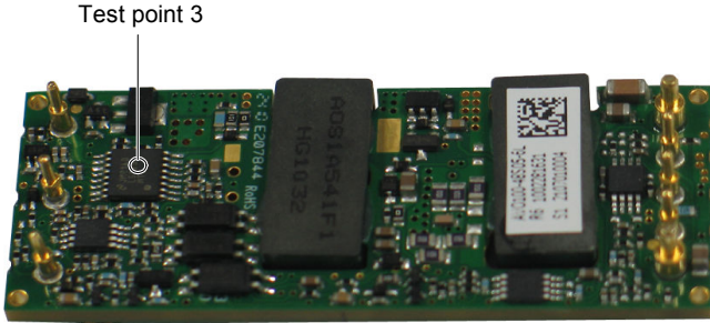
Figure 16 Temperature test point on converter
