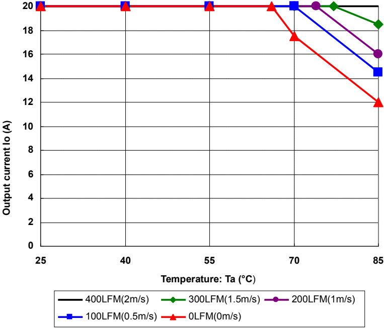
Figure 17 Derating curve
