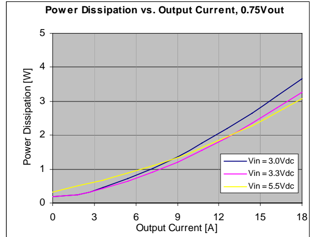
Figure 5. Power Dissipation vs. Load Current at ambient temperature, T_A = 25^\circ\text{C} .
