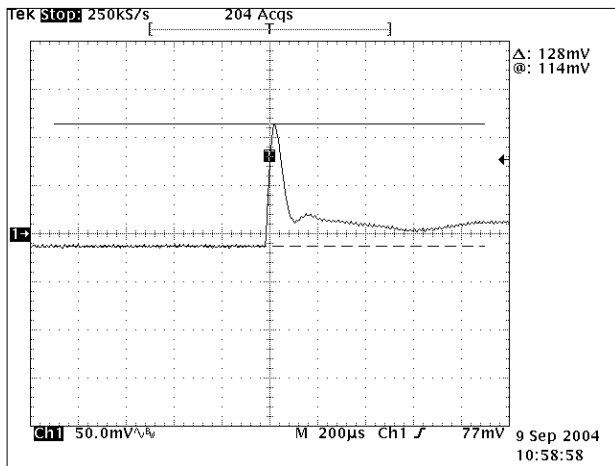
Figure 22. 2V5 Output Transient Response (100% to 50% I_{omax} ) at V_{in} = 3.3V , T_A = 25^\circ C .
