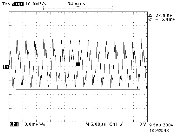
Figure 20. 2V5 Output Ripple Waveform at V_{in} = 5.5V , I_{out} = 18A , T_A = 25^\circ C .
