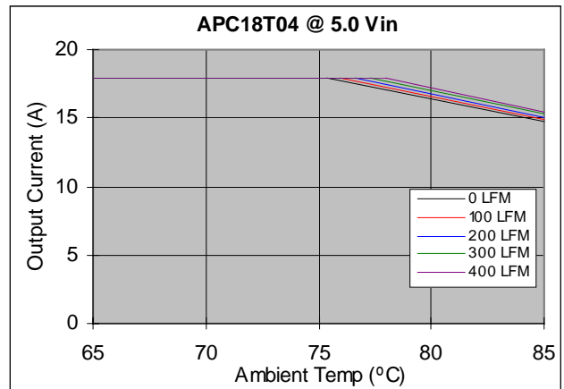
Figure 11. Output Power Derating Curve for 0.75V_{OUT} at V_{IN} = 5V , T_A = 25^\circ\text{C}
