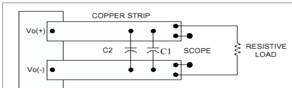
Figure 2. Peak-to-Peak Output Noise Measurement Test Set-up
