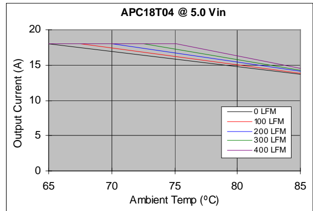
Figure 13. Output Power Derating Curve for 1.8V OUT at V IN = 5V, T A = 25°C
