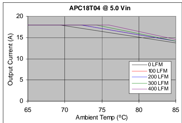
Figure 15. Output Power Derating Curve for 3.3V OUT at V IN = 5V, T A = 25°C
