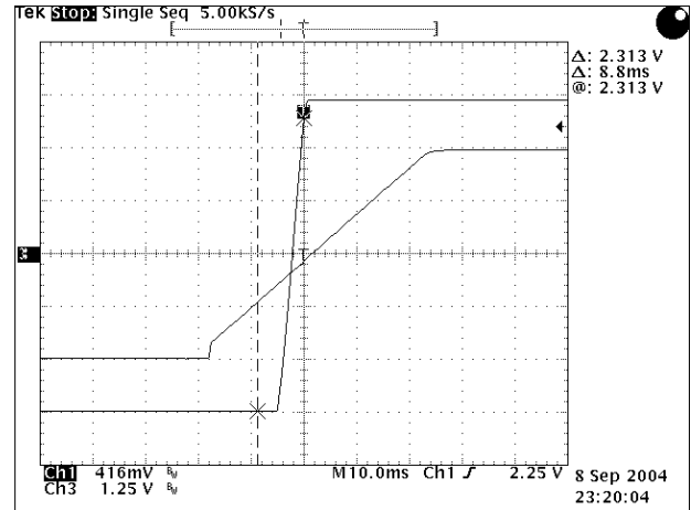
Figure 21. 2V5 Output Enable Turn On Characteristic at V_{in} = 3.3V , T_A = 25^\circ C .
