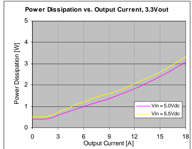
Figure 9. Power Dissipation vs. Load Current at ambient temperature, T_A = 25^\circ\text{C}
