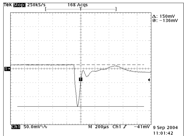
Figure 23. 2V5 Output Transient Response (50% to 100% I_{omax} ) at V_{in} = 3.3V , T_A = 25^\circ C .
