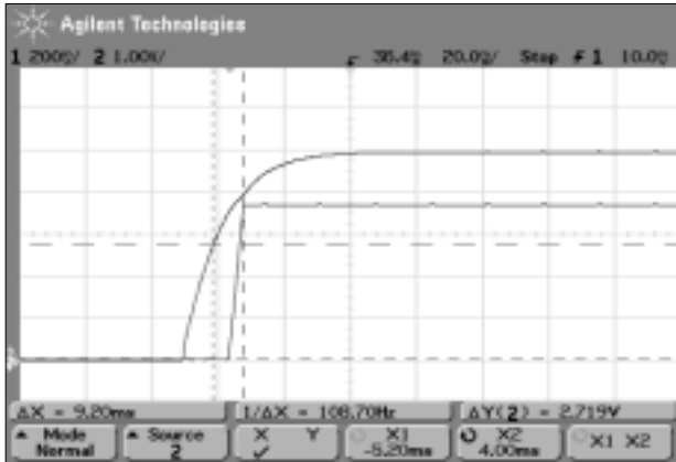
Figure 16. Output Startup Waveform for 0.75V OUT at V IN = 5V, I OUT = 18A.
