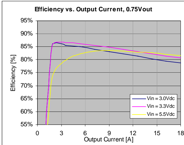
Figure 4. Efficiency vs. Load Current at ambient temperature, T_A = 25^\circ\text{C} .
