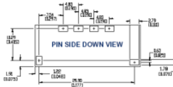
Figure 24. Mechanical Outline
