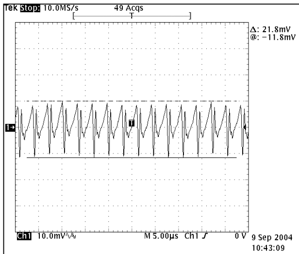
Figure 18. 2V5 Output Ripple Waveform at Vin = 3V, Iout = 18A, T A = 25°C.
