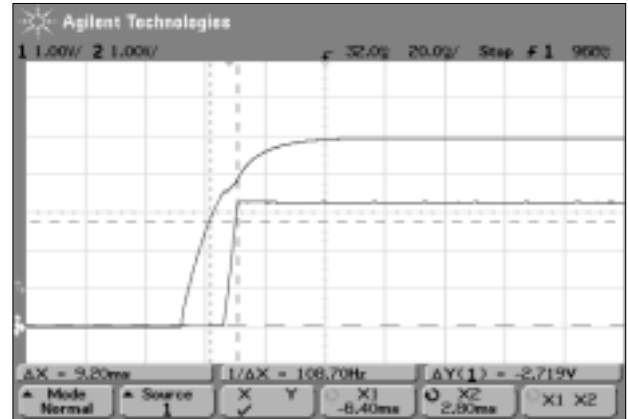
Figure 17. Output Startup Waveform for 3.3V OUT at V IN = 5V, I OUT = 18A.
