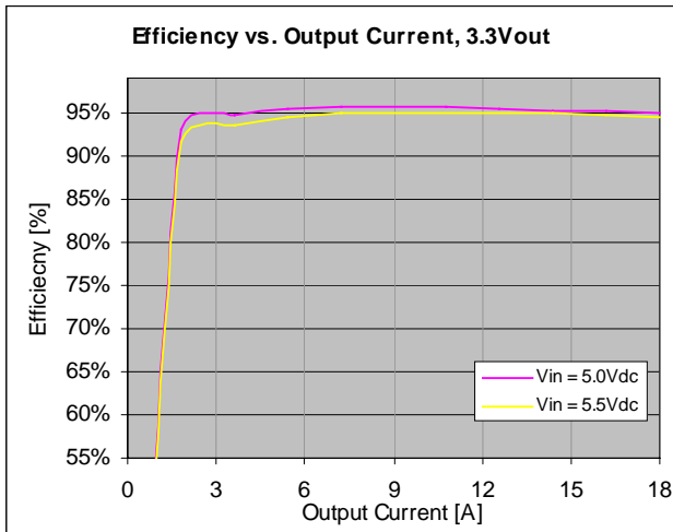
Figure 8. Efficiency vs. Load Current at ambient temperature, T_A = 25^\circ\text{C} .
