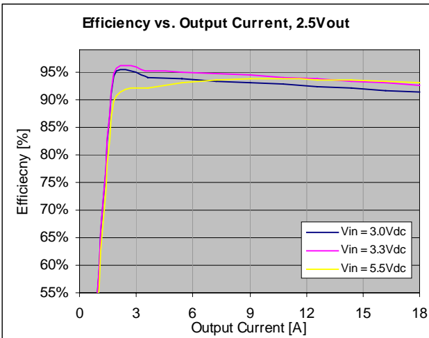
Figure 6. Efficiency vs. Load Current at ambient temperature, T_A = 25^\circ\text{C} .
