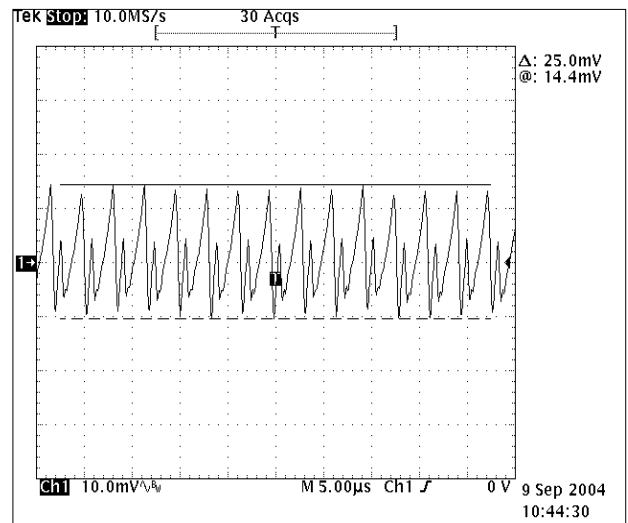
Figure 19. 2V5 Output Ripple Waveform at Vin = 3.3V, Iout = 18A, T A = 25°C.
