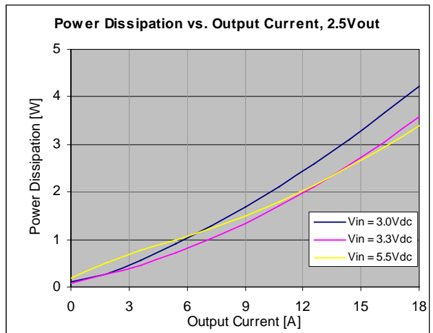
Figure 7. Power Dissipation vs. Load Current at ambient temperature, T_A = 25^\circ\text{C} .
