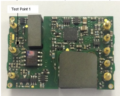
Figure 12 Temperature test point(Bottom)
