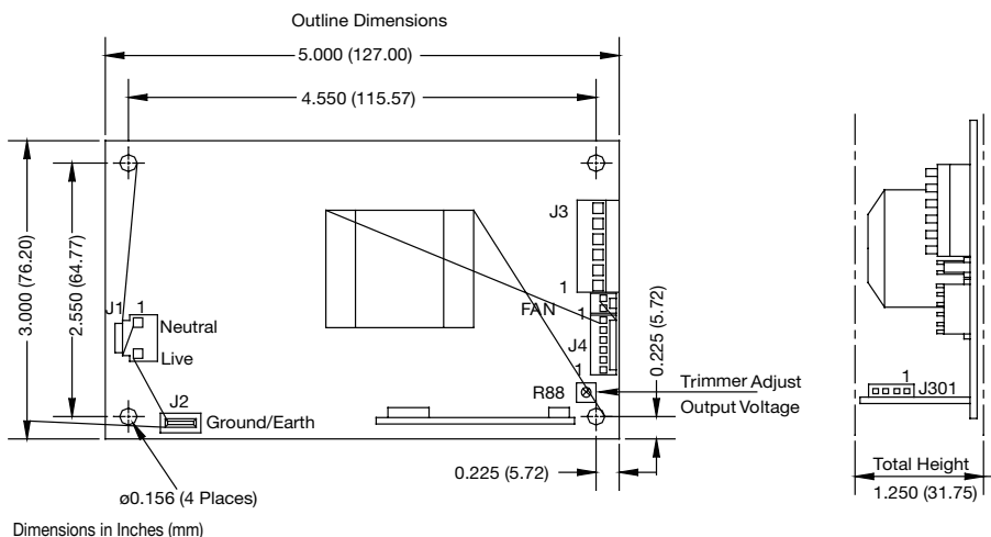
Figure 2: Mechanical Drawing
