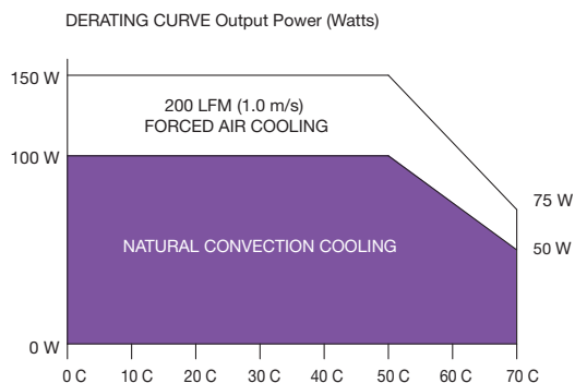
Figure 1: Derating Curve
