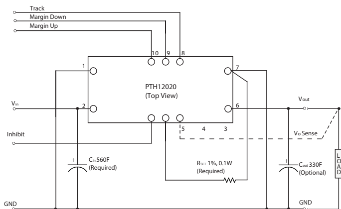
Figure 8 - Standard Application
