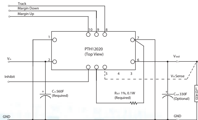
Figure 5 - Standard Application
