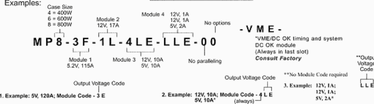
Dual Output 3-digit Code Selection Chart
