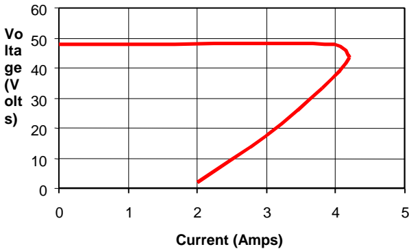
1W Output Current Limit (48V 4A)
