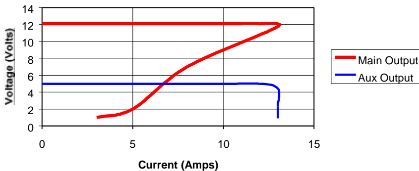
4LE Output Current Limit (12V 10A & 5V 10A)
