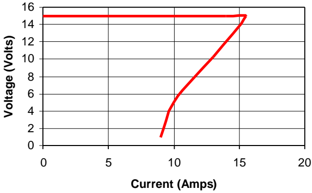
1N Output Current Limit (15V 14A)
