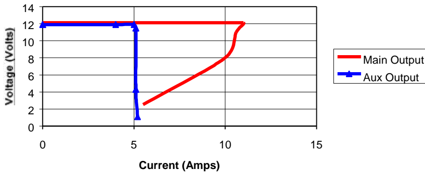
4LL Output Current Limit (12V 10A & 12V 4A)
