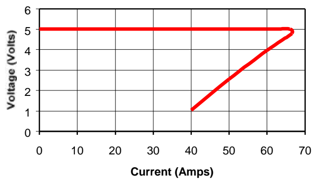
2E Output Current Limit (5V 60A)
