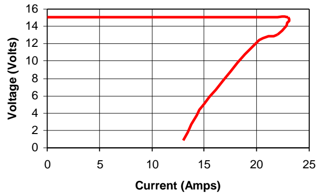
2N Output Current Limit (15V 20A)
