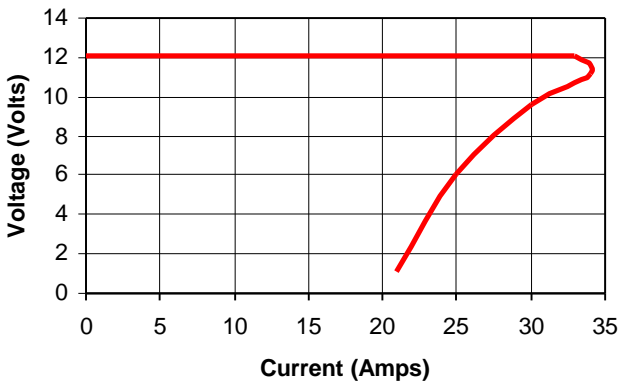
2L Output Current Limit (12V 30A)
