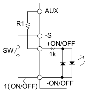
Figure 15 Connection of remote ON/OFF control (B)
