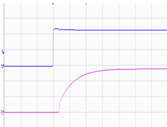
Figure 8 Output voltage startup by power on, (20ms/div), see Figure 13 for test configuration, CH1-input voltage (10V/div); CH2-output voltage (10V/div)
