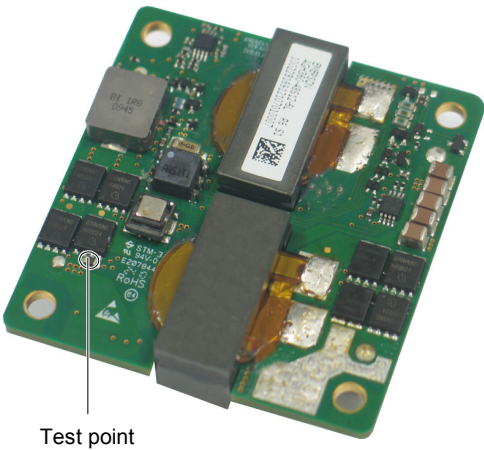
Figure 10 OTP test point
