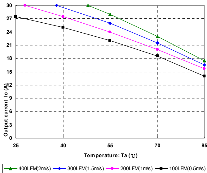
Figure 18 Output power derating, 48Vin, air flowing across the converter from pin 1 to pin 3
