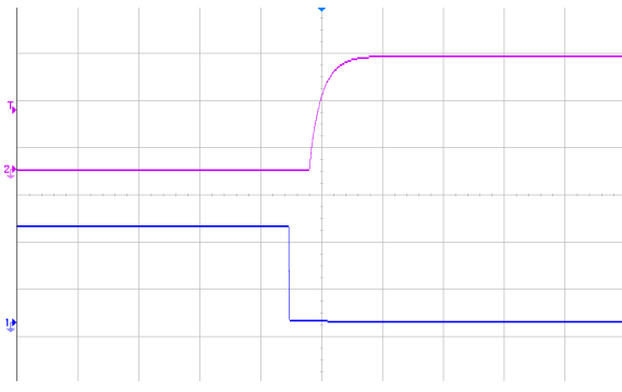
Figure 8 Output voltage startup by remote ON, (50ms/div), see Figure 11 for test configuration; CH1-remote ON (2V/div); CH2-output voltage (5V/div)
