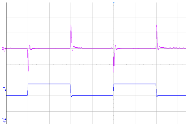
Figure 4 Dynamic response for 25% load step (50% ~ 75% ~ 50%) and 0.1A/ \mu\text{s} slew rate, (2ms/div), see Figure 11 for test configuration; CH1-output current (10A/div); CH2-output voltage (200mV/div)
