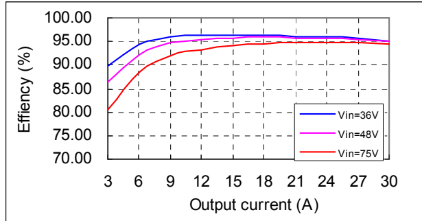
Figure 1 Efficiency vs. output current, T_a=25^{\circ}\text{C} , 400LFM, V_o=12\text{V}
