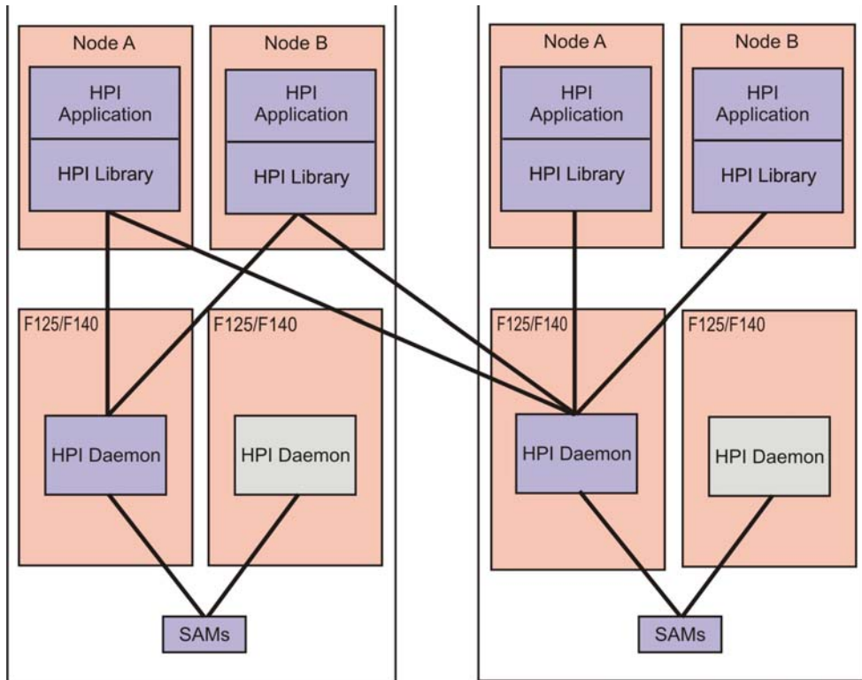
Figure 1-1 Overview of HPI Usage in Systems
