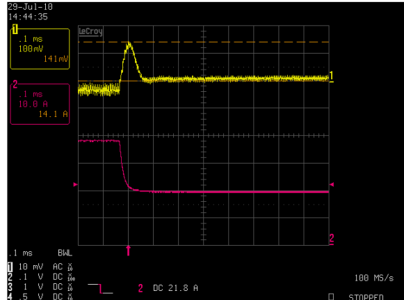
Figure 8: DS460S-3-002 Transient Response – Vo Deviation (high to low) 100% to 50% load change, 1A/ \mu S slew rate, Vin = 230Vac Ch 1: Vo Ch 2: Io
