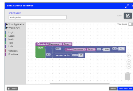
The PowerPro GUI incorporates a powerful script creator function that allows users to write their own process control routines.
